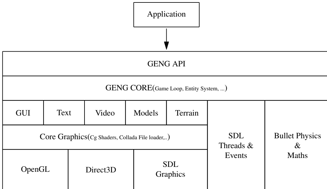
Figure 1. Geng Architecture
